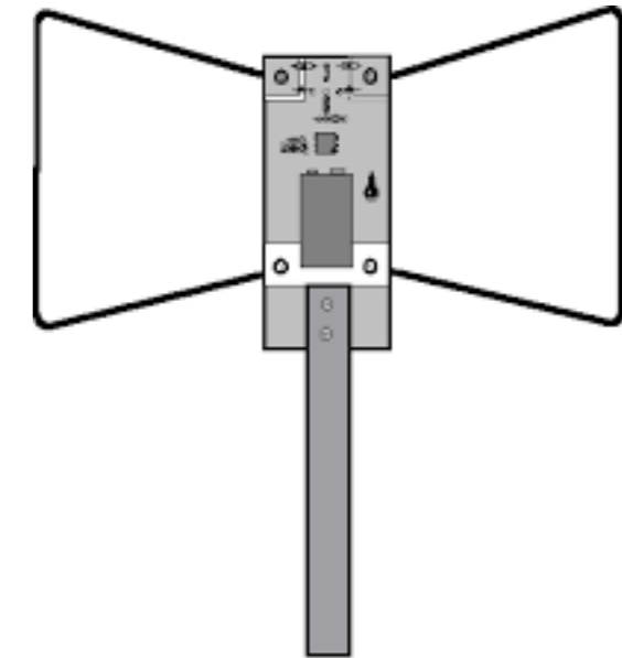
Fig. 1 - The assembled TDOA antenna unit - coaxial cables to receive runs behind the PCB and through the PVC pipe handle.
